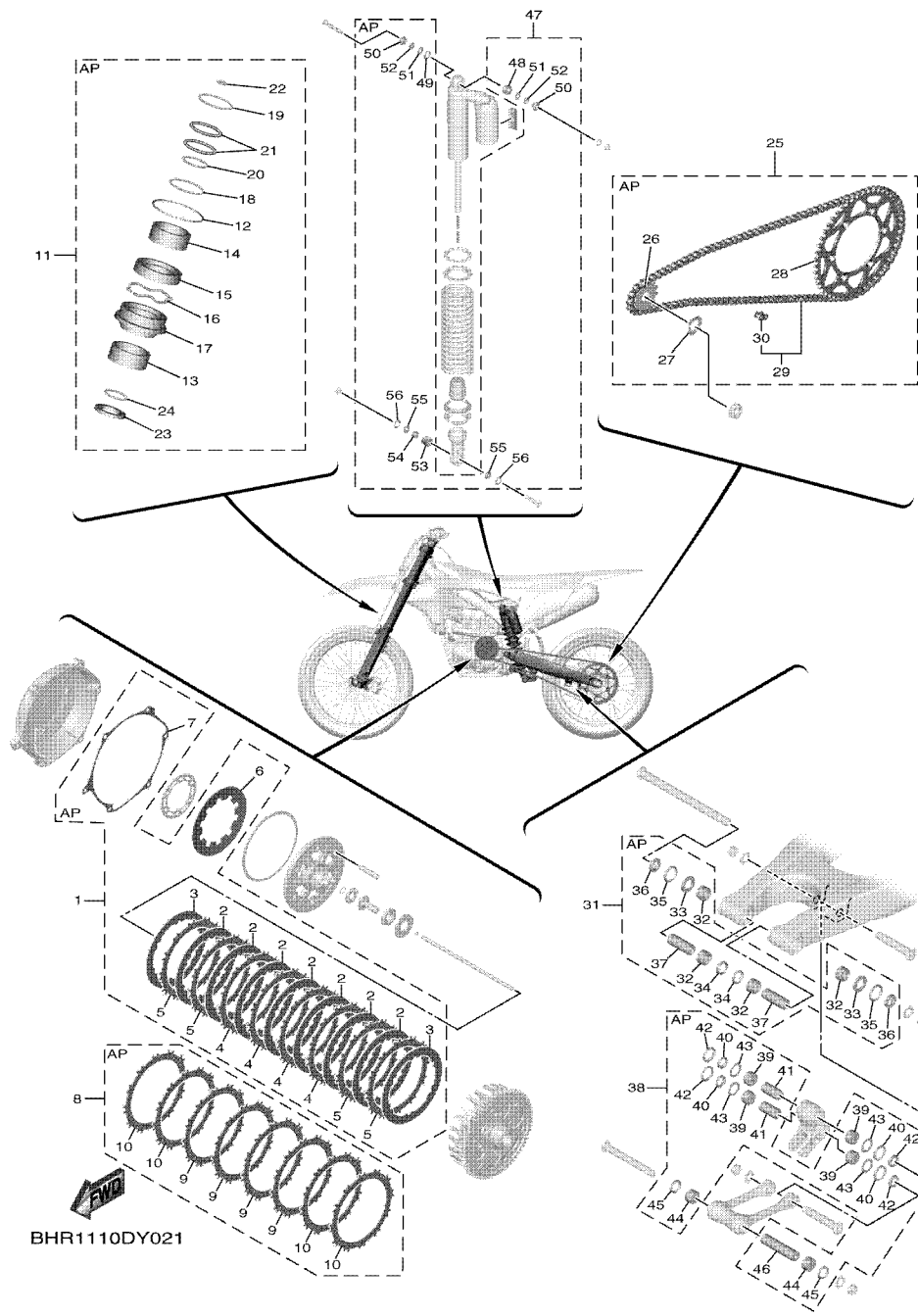
FIG. 2 MAINTENANCE PARTS KIT
